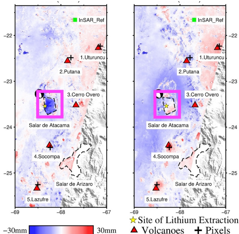
Figure 1. InSAR derived descending line-of-site displacements (left panel: 2018-2020; right panel 2020-2022) in the Atacama region of northern Chile showing deformation in the Salar de Atacama (magenta box). A major centre of Li extraction is indicated by the yellow star. Adapted from Liu et al., 2023. ( https://doi.org/10.1029/2022GL102480 )
