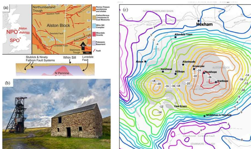
Figure 1: (a) Simplified geological map and schematic north-south cross-section of the Alston Block based on the line of section (white). Source of image a - https://www.lyellcollection.org/doi/full/10.1144/jgs2020-226 ; (b) Groverake Mine is near Rookhope in Weardale in the North Pennine Orefield and (c) a Bouguer Gravity Anomaly map reveals the contours of granite mass below the North Pennine Orefield in close relationship to the fluorite zone and major ore seams. Source of images b and c - https://www.geologynorth.uk/north-pennine-orefield/
